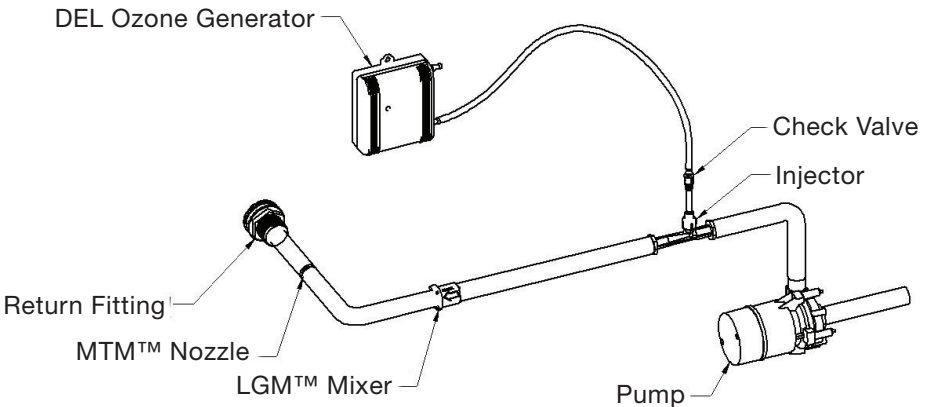
DEL Optimized Mixing System
